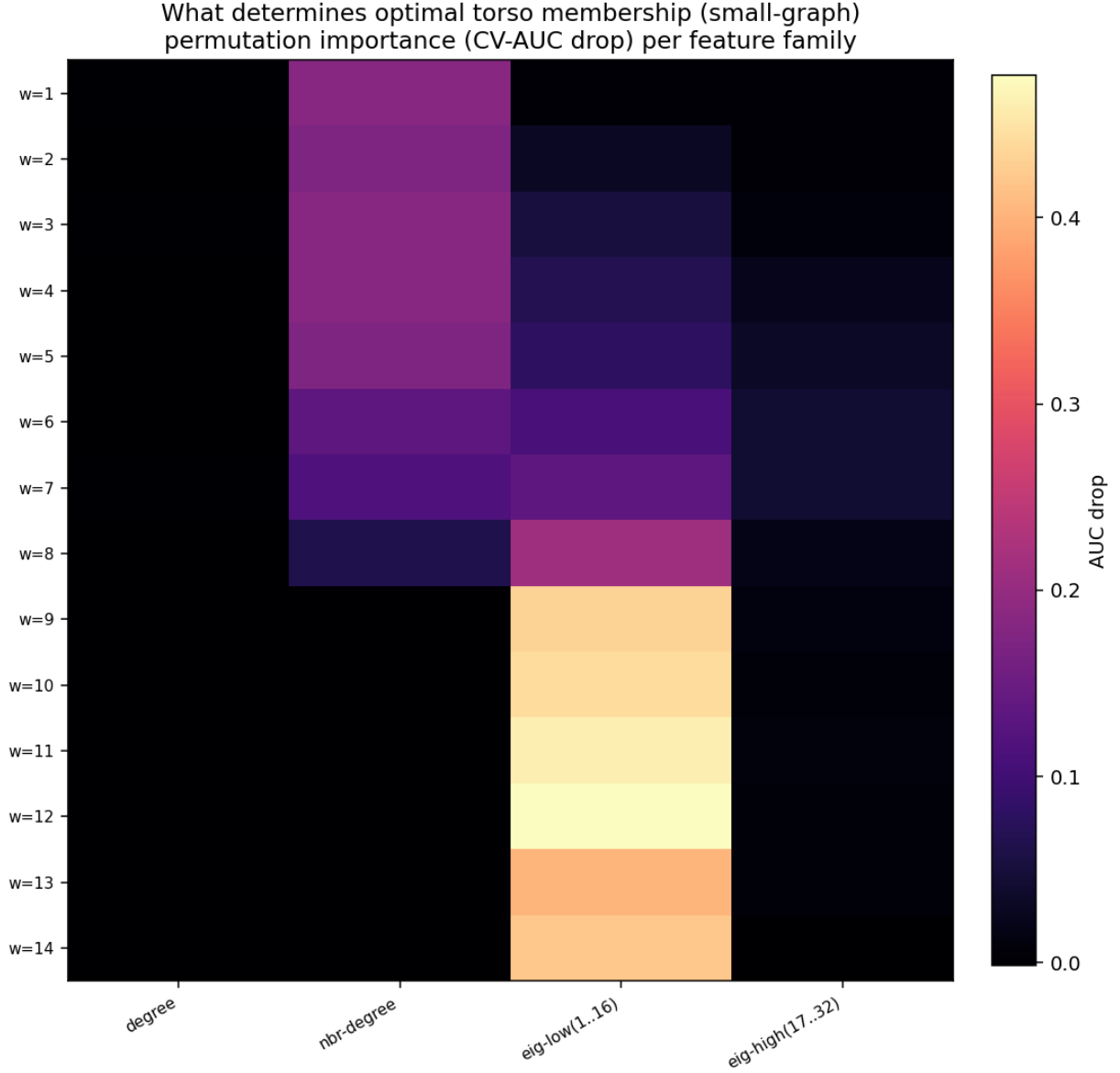
Figure 14: GBDT permutation-importance map of optimal torso membership (small-graph). The determining signal hands off from the local neighbour-degree column (bands 1–7) to the low-Laplacian-eigenvector column (bands 8–14) exactly at the band-8 boundary — the same boundary at which the +6 HV gap and the clique obstruction live.
